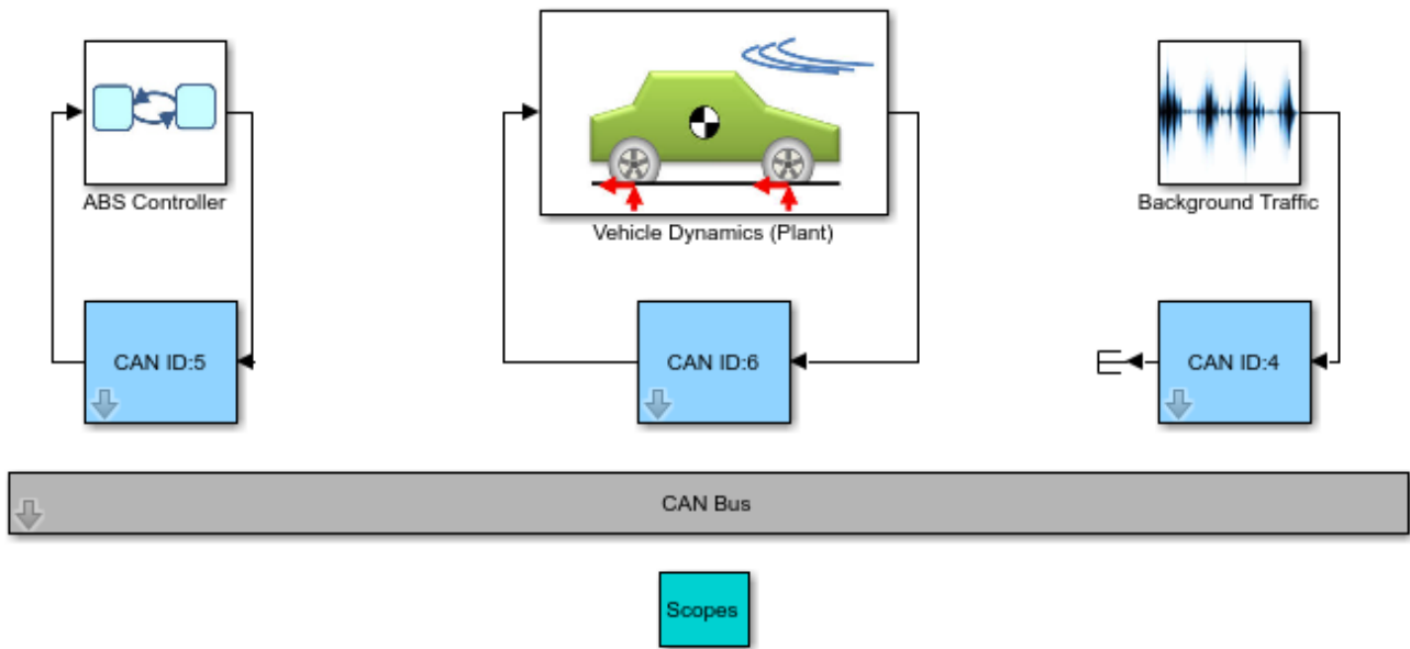
Effects of Communication Delays on an ABS Control System
